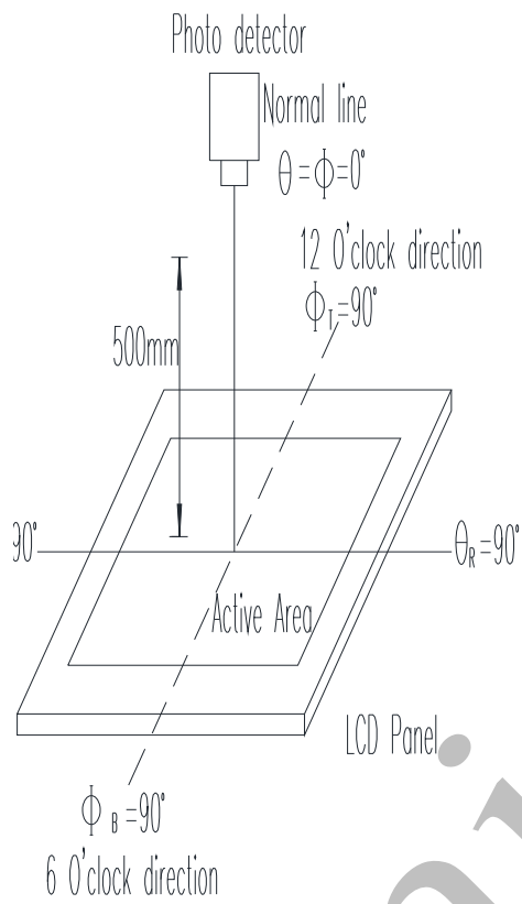
Fig. 9.2. Optical measurement system setup
